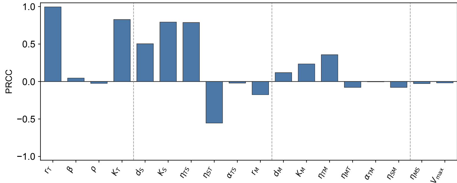
OVCAR4: PRCC on AUC of Tumor cells T(t) | Tumor+MSC+M2
